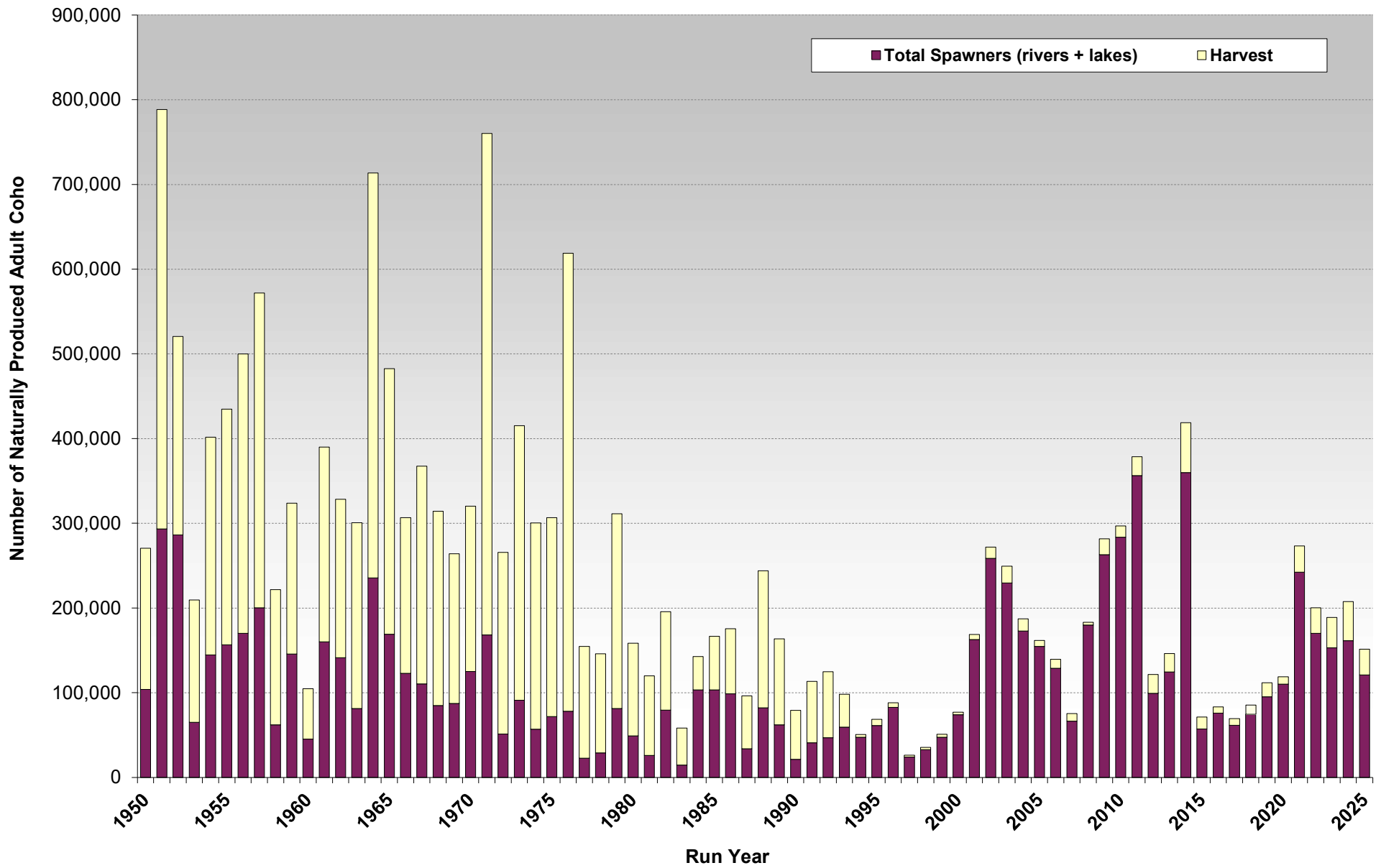
Estimate of naturally produced adult coho in the Oregon Coast Coho ESU (run years 1950 to 2025). Number of adult coho spawning in the wild, and harvest impacts (both landed and non-landed).
